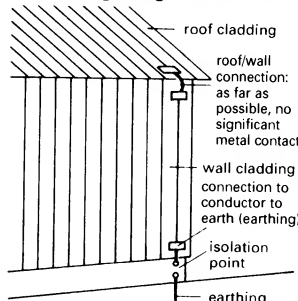
⑤ Aluminium wall cladding used as a conductor to earth
